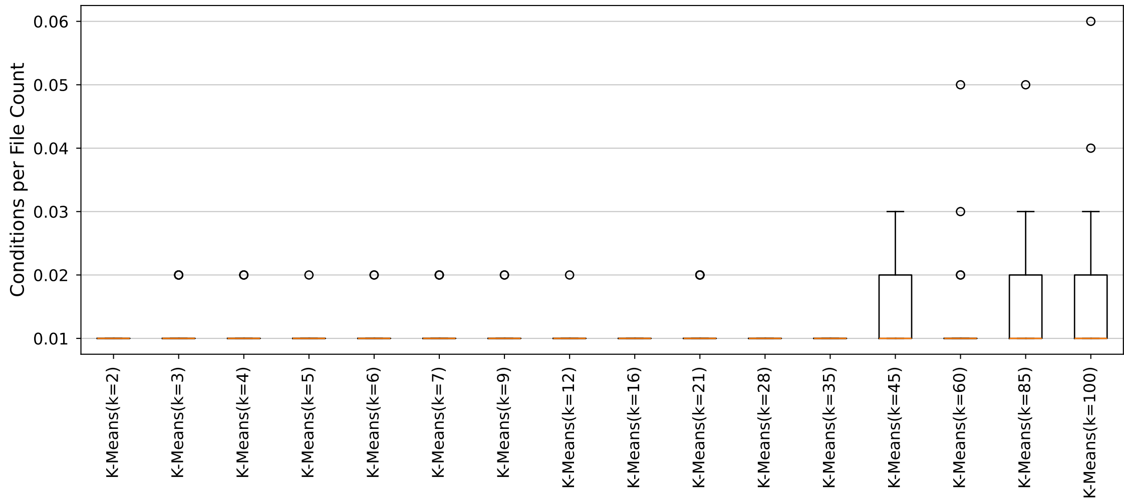
YARA Rules Conditions per File Count Distribution (Cluster2_Size100 dataset)
